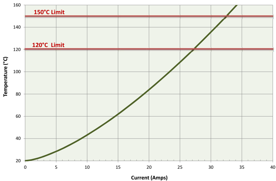
125-25 High Current Series (125-PRH2509H with 125-SDH250S)
