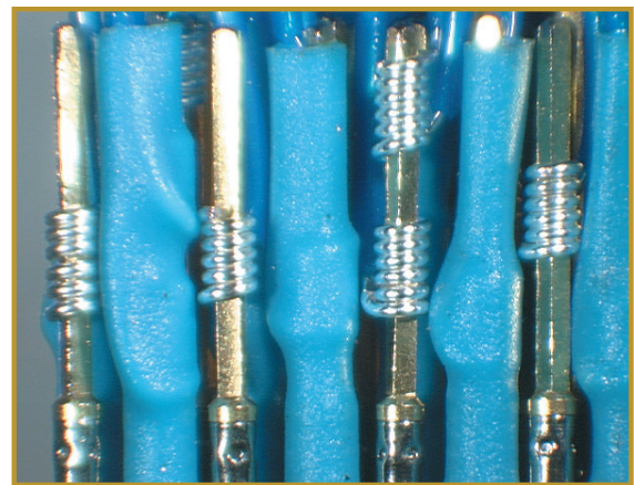
Finished assembly showing heat shrunk insulating tubing on alternate posts.
