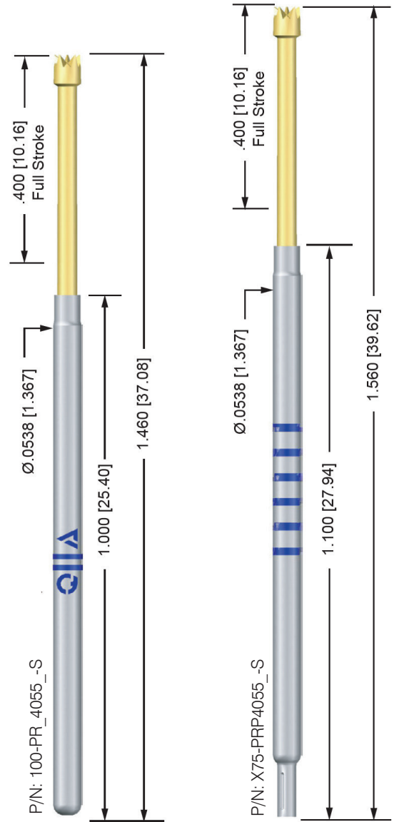
.400 [10.16] Full Stroke, .317 [8.05] Working Stroke
